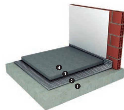
1- floor slab 2- fonomix 15/40 n 3- mortar screed 4- floor tile
