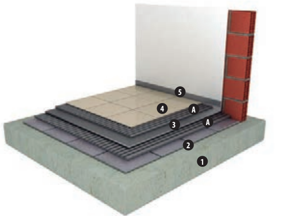
1- floor slab 2- old floor tile 3- fonopac R eco 4- floor tile 5- bandin A- cement-based adhesive
