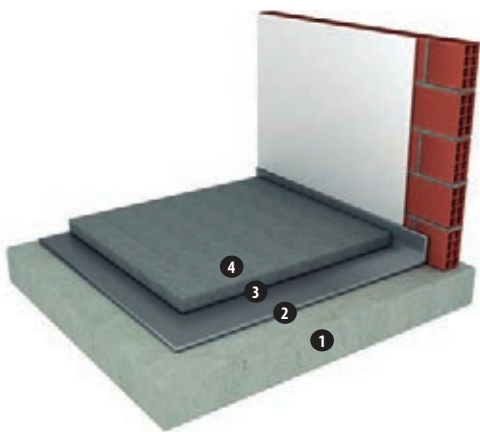
1- floor slab 2- fonos (+) 3- mortar screed 4- floor tile
