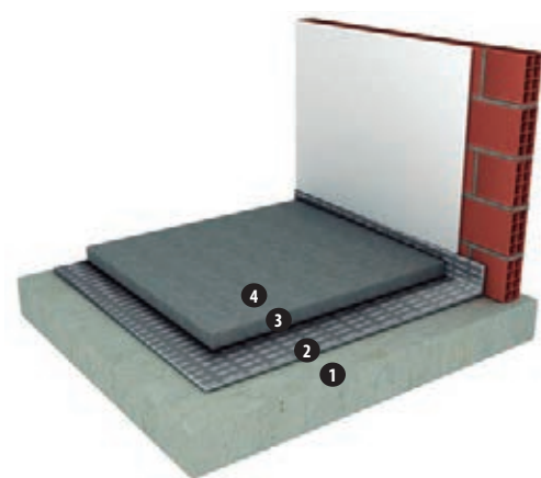
1- floor slab 2- fonomix 15/15 n 3- mortar screed 4- floor tile
