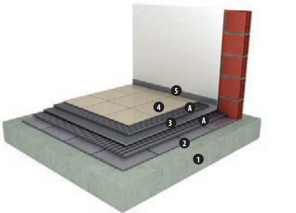
1- floor slab 2- old floor tile 3- fonopac R 4- floor tile 5- bandin A- cement-based adhesive + fonolax
